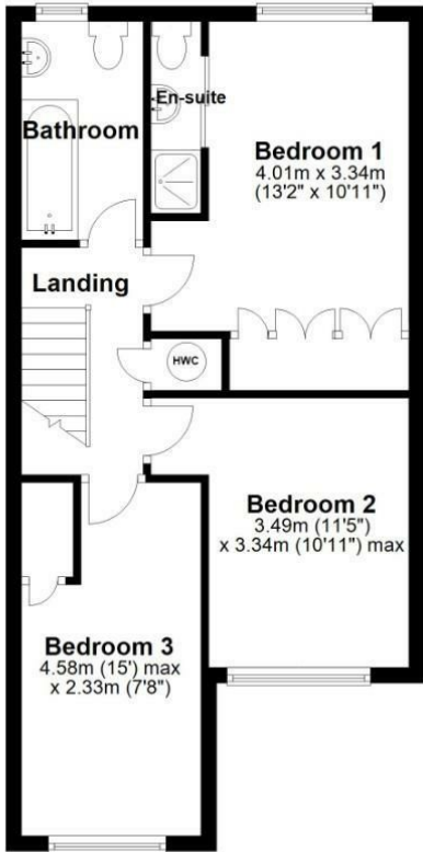
First Floor Approx. 47.8 sq. metres (514.2 sq. feet)
